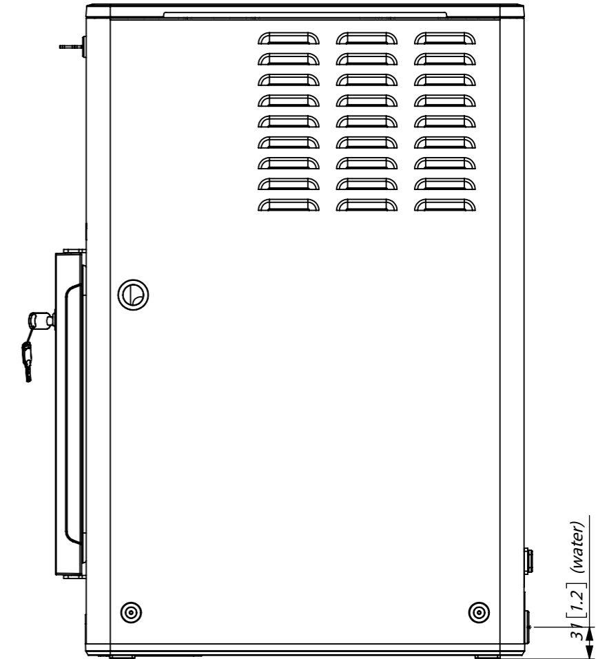
Right
