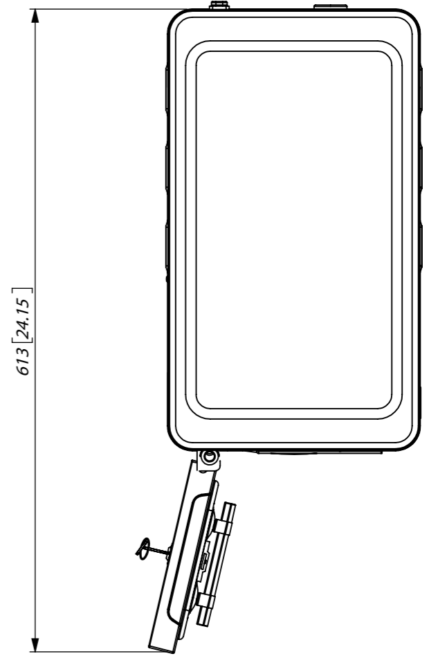
Right
